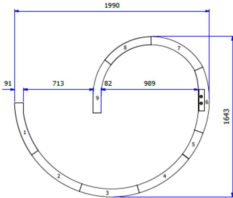
PLAN (1990 W x1643 L x 2170 H)
